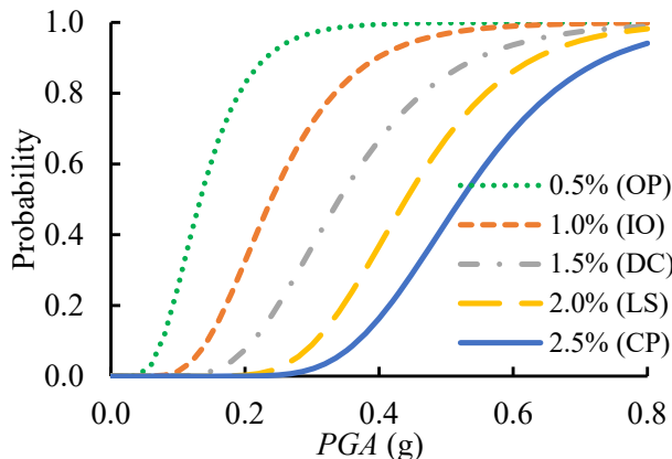
Fig. 1. Fragility curves of the target building in X-direction. Each line corresponds to five different performance level range. Similar curves are also developed for Y-direction of the target building.
