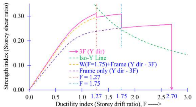
Fig. 2. Performance improvement by improving the deformation behavior after considering the infill wall (Third floor in Y direction is shown as an example).
